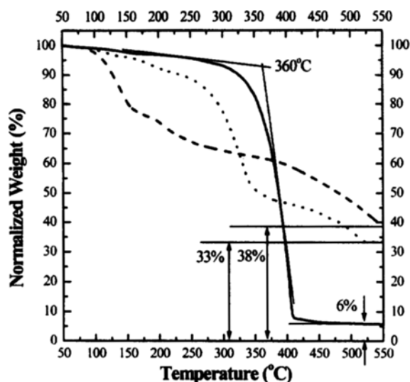
Fig. 1. Thermogravimetric analysis of fresh Ba(DPM) 2 (—), aged Ba(DPM) 2 stored for 3 months (···) or for 6 months (---) in a desiccator.
